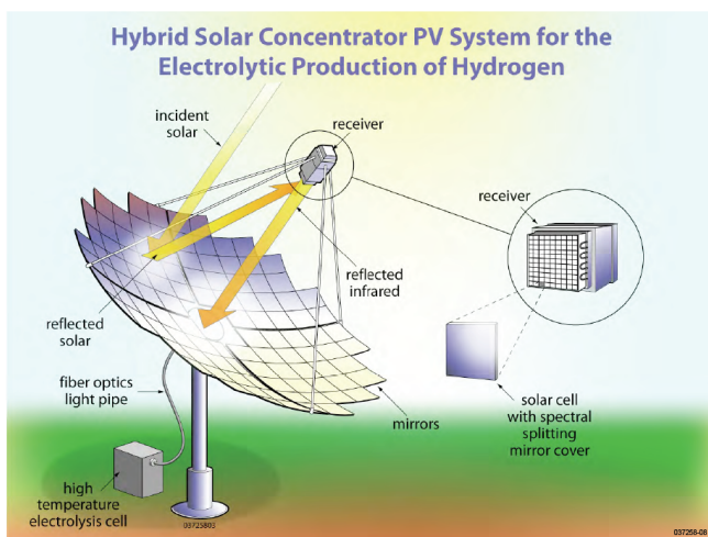
Figure 1: SCPV combined with HTCE system
