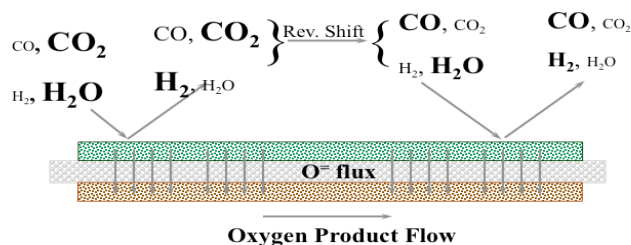
Figure 2: HTCE mechanism
